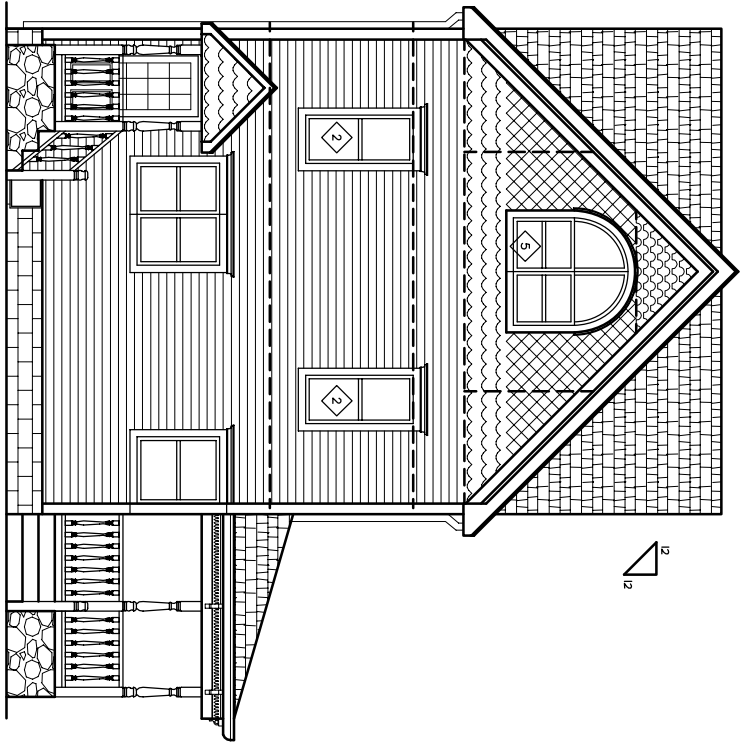
SOUTH ELEVATION 1/4" = 1'-0"
