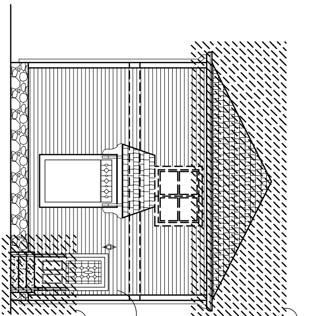
DEMOLITION NORTH ELEVATION 1/4" = 1'-0"
