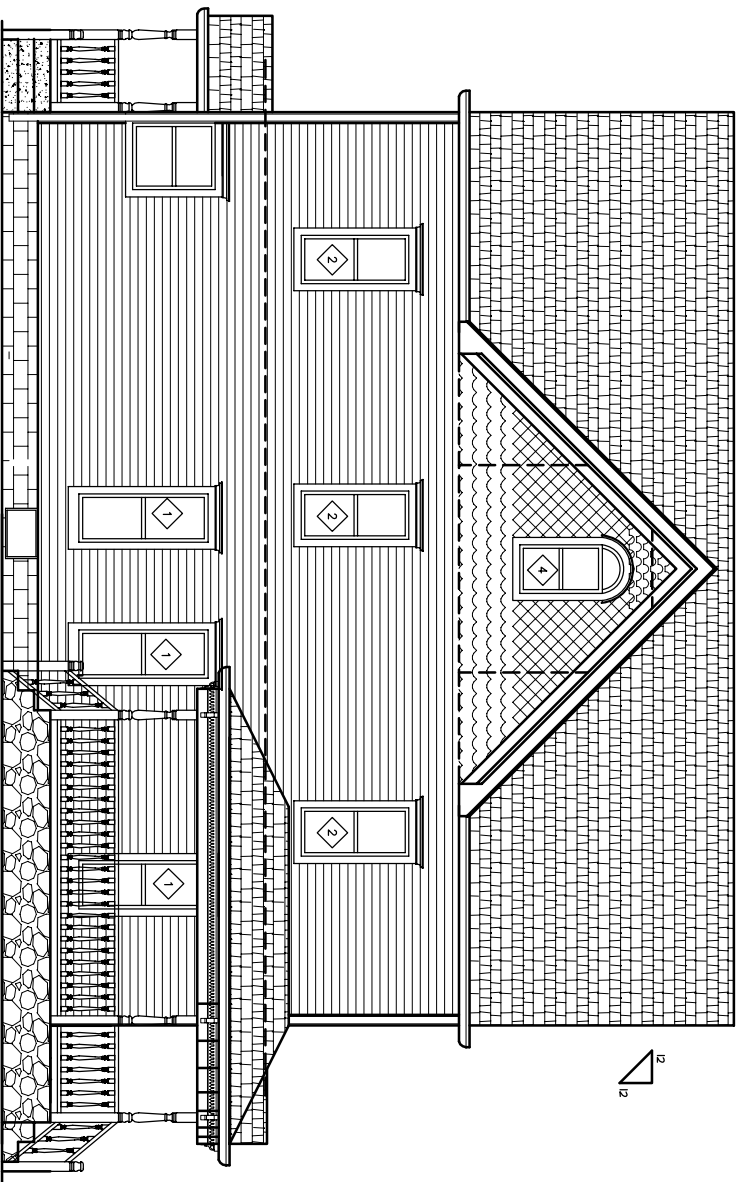
EAST ELEVATION 1/4" = 1'-0"
